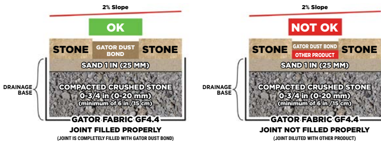
Sand or ASTM No. 9 Stone can be used as a bedding layer
