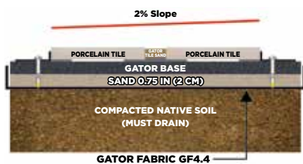
Option 3a • Porcelain Tile on Gator Base
